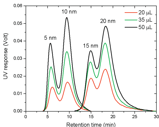
Figure 2: UV-based fractograms combined for mixtures of 5 nm/10 nm and 15 nm/20 nm AuNPs, using a regenerated cellulose membrane in the AF4 channel.
