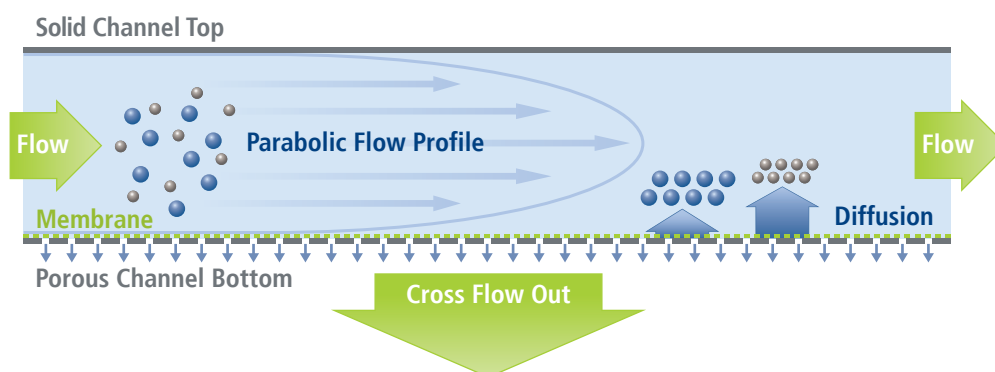
Figure 1: Schematic for the AF4 separation principle.
