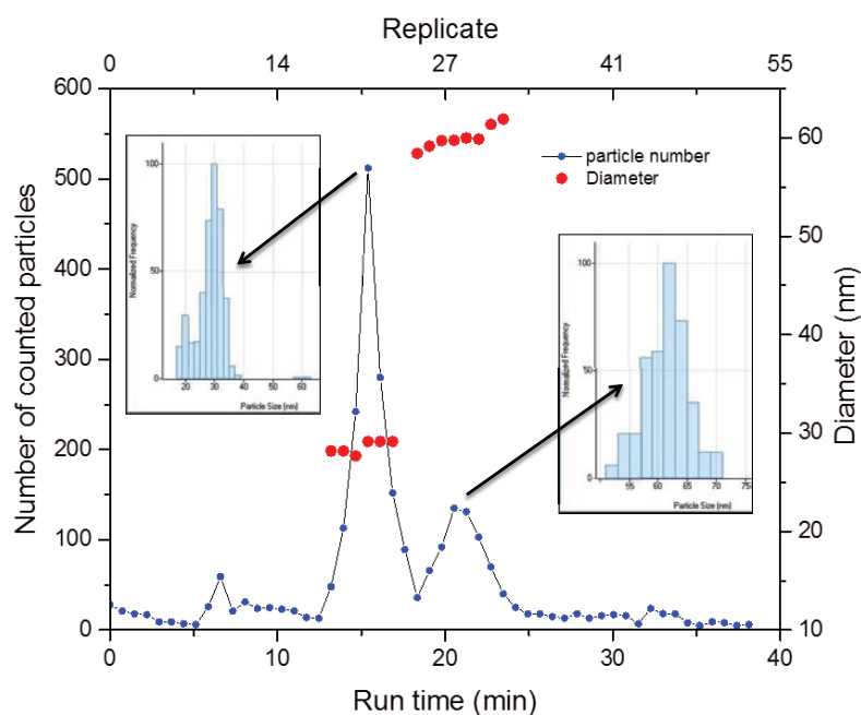
Figure 2. Particle number-based fractogram of the mixture of 30 nm and 60 nm Au gold nanoparticles obtained by AF4-splCP-MS. The red circles represent the average replicate diameter measured by splCP-MS. The shown histograms representing the particle size distribution at the respective peak maxima are directly obtained from the Agilent MassHunter Workstation software.
